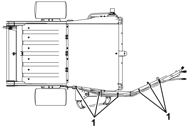
Figure 12 Front View
