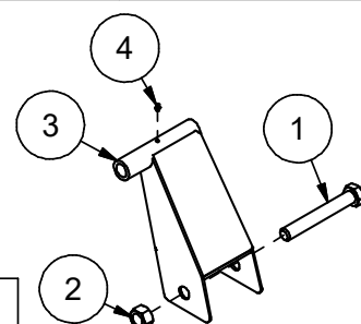
Riser, Offset XRM, Left 205349
